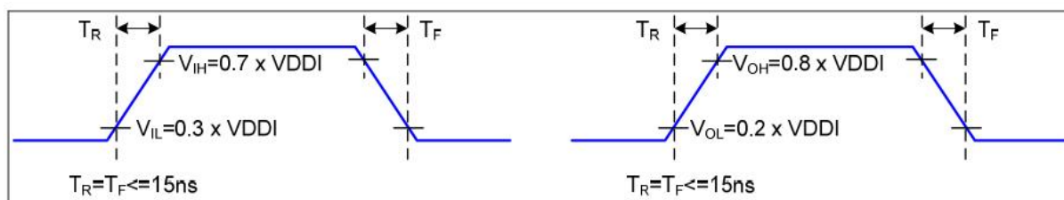
I/O 信号的上升和下降时序 Rising and Falling Timing for I/O Signal
